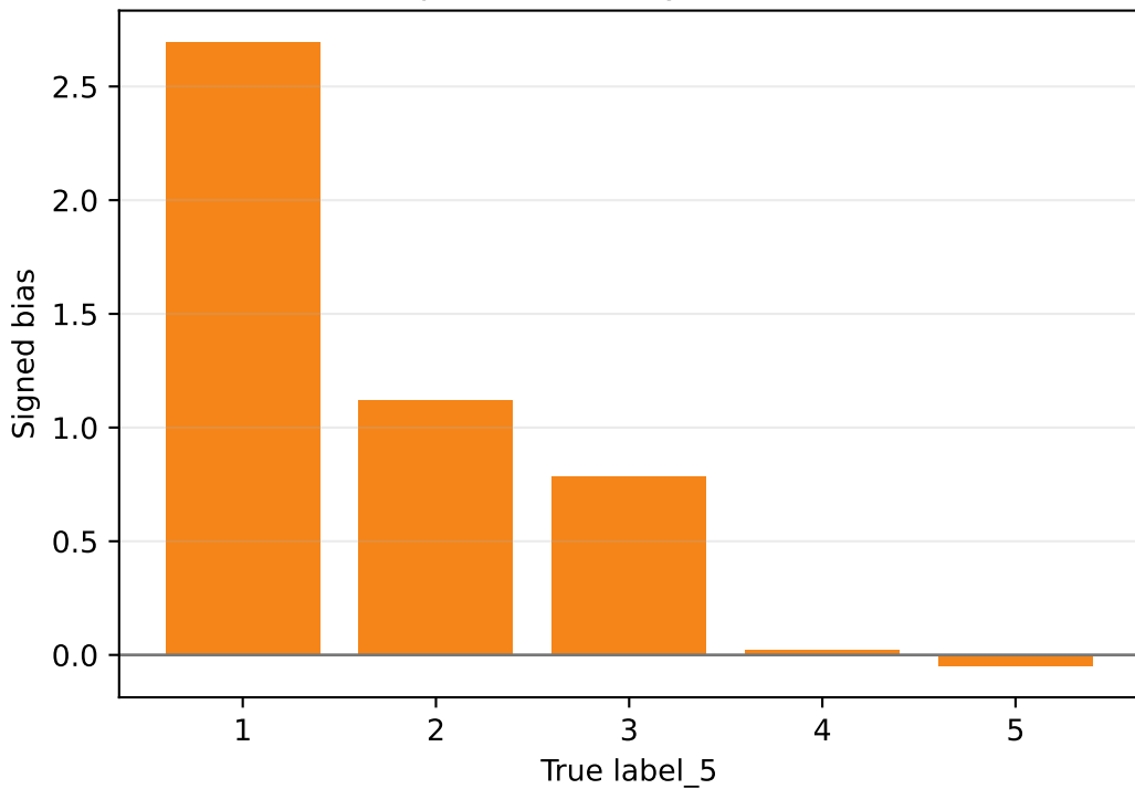
Exp2 Test Bias by True Score
