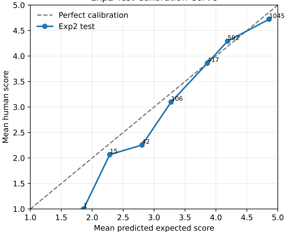
Exp2 Test Calibration Curve
