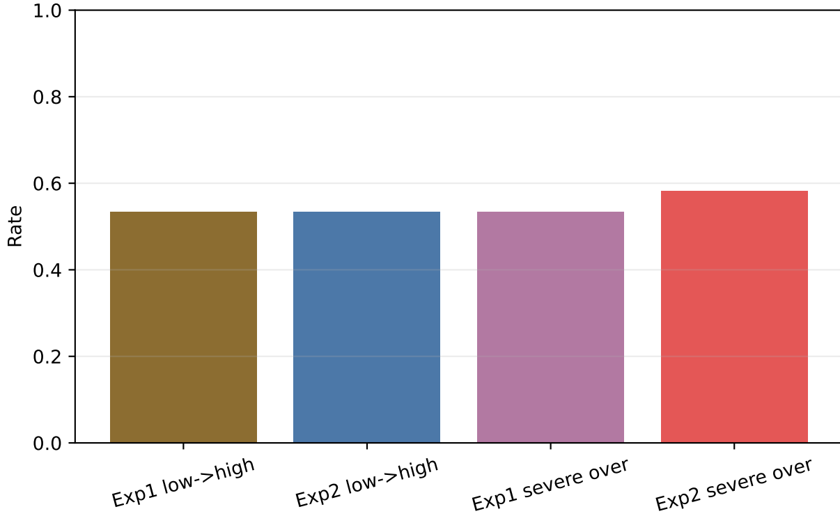
Low-Score Overestimation Remains the Main Failure Mode
