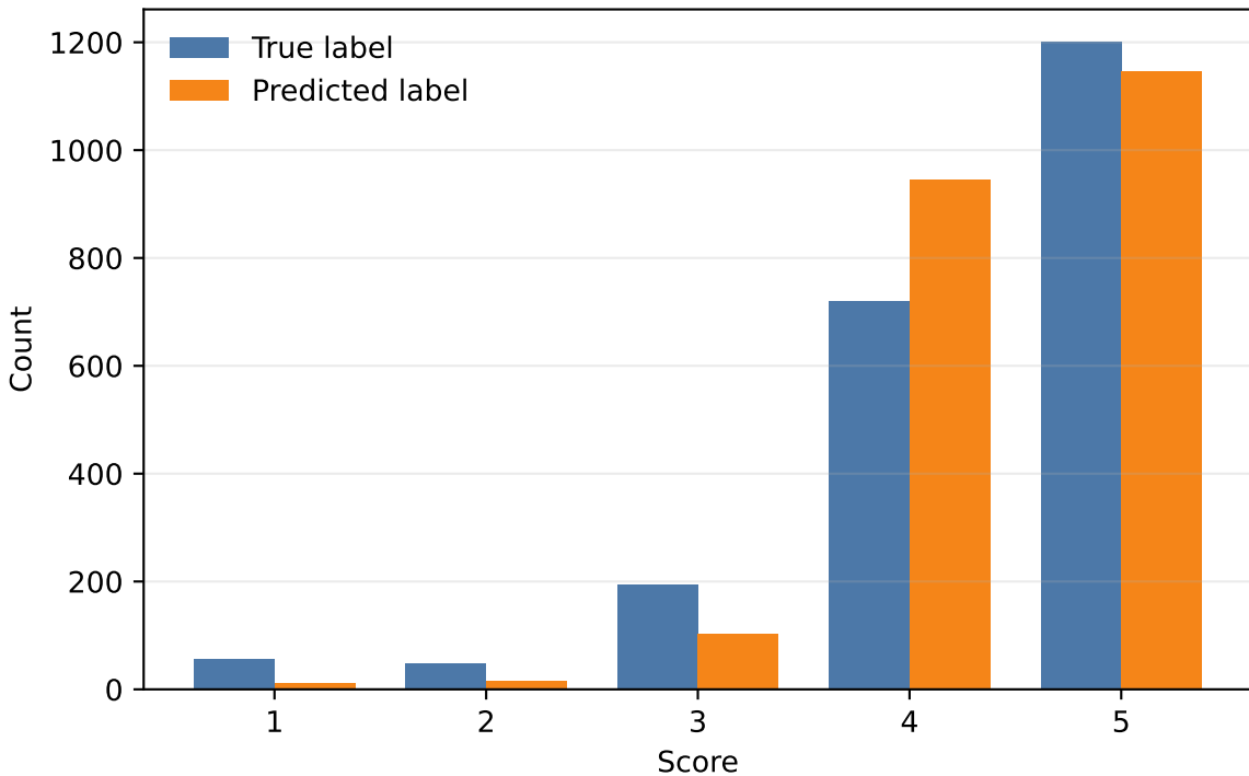
Exp2 Test Predicted vs True Score Distribution
