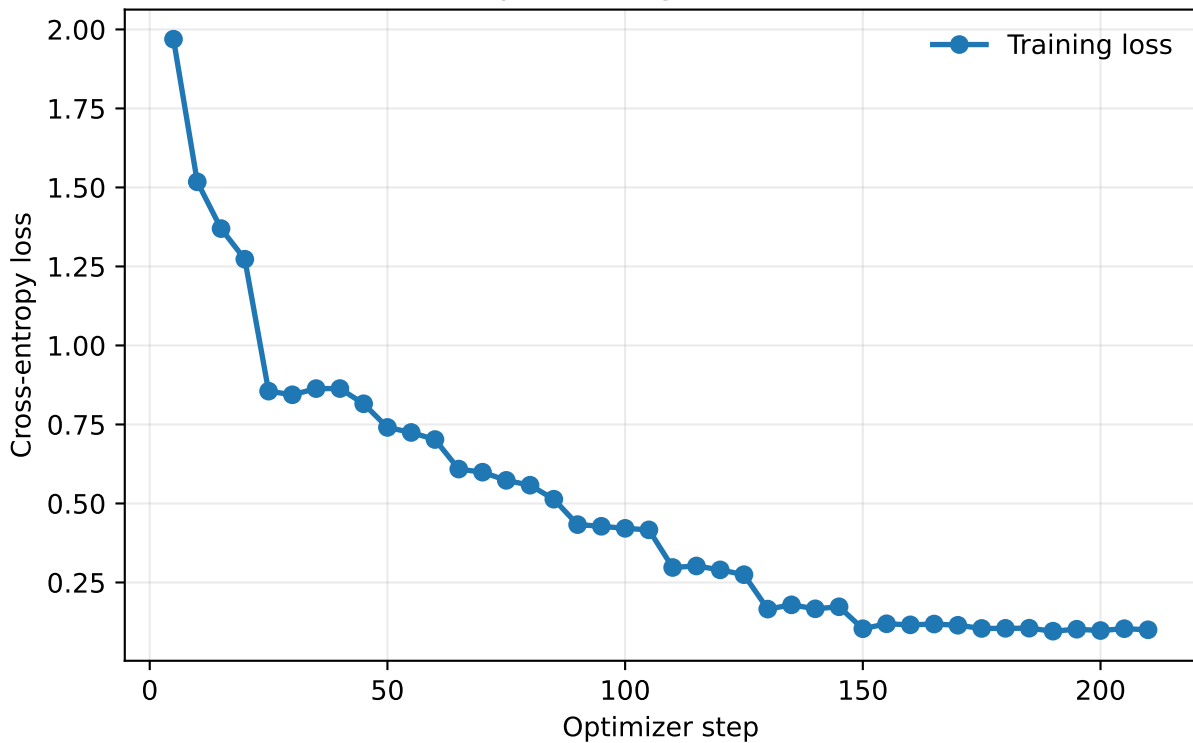
Exp2 Training Loss Curve
