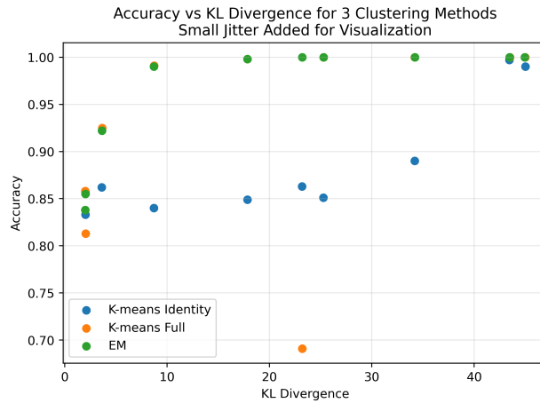
Figure 4: Accuracy vs. KL Divergence for the 3 methods on the 10 runs. Small jitter added to x values for visualization.
