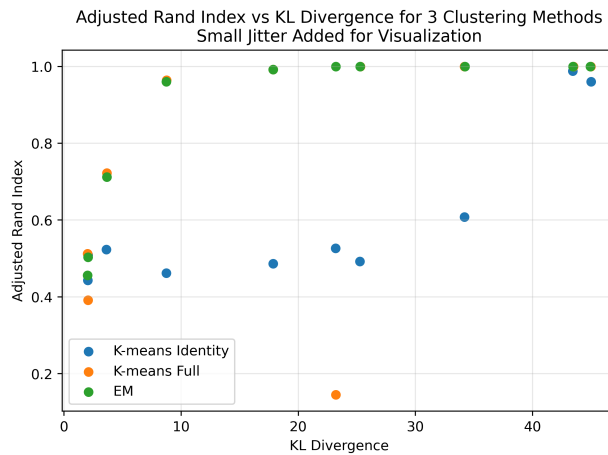
Figure 5: Adjusted Rand Index vs. KL Divergence for the 3 methods on the 10 runs. Small jitter added to x values for visualization.
