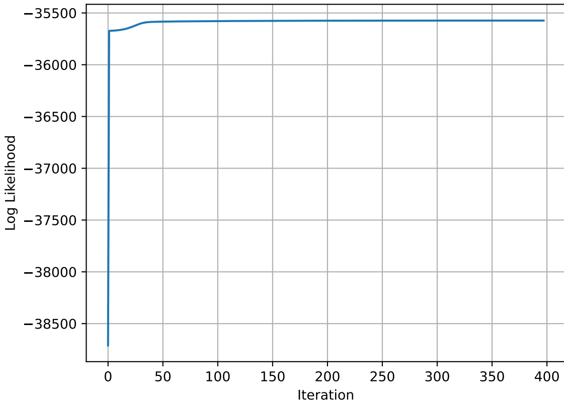
Baum-Welch Log-Likelihood Trace (tol=0.001)
