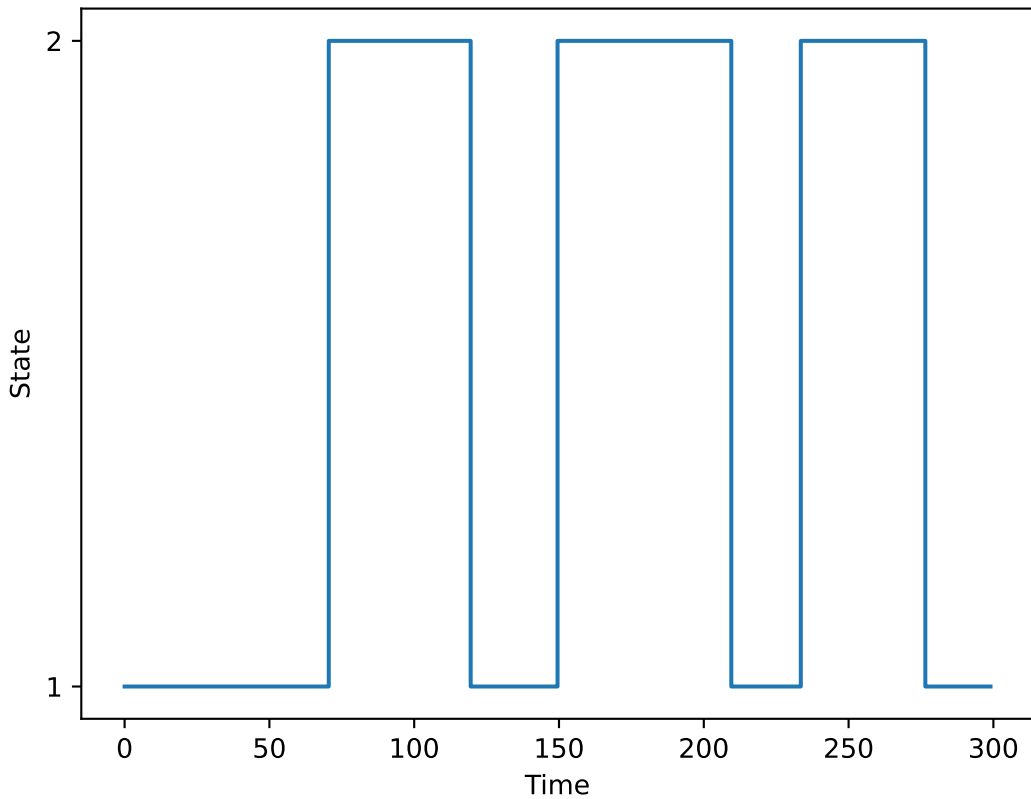
Most Likely Hidden State Sequence (Viterbi)
