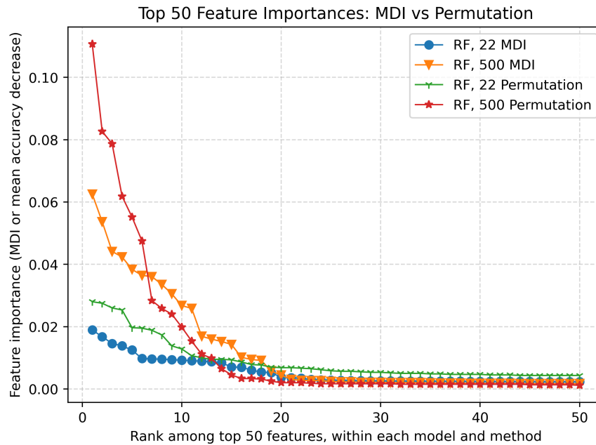
Figure 1: Feature Importances for the two RF, computed via MDI and via Permutations
