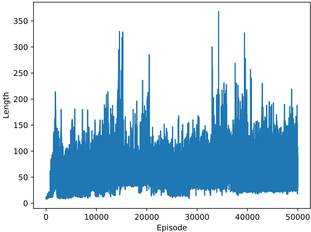
Episode Length vs Episode (N=50000)
