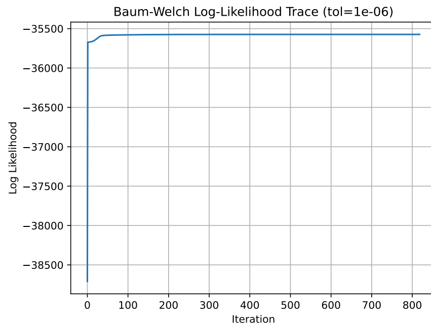
Figure 2: Log Likelihood of Baum Algorithm, showing convergence.
