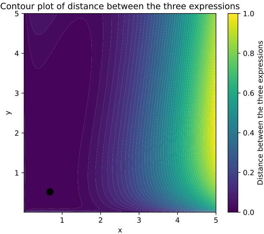
Figure 1: Distance between the three equations and what x, y value minimizes said distance.
