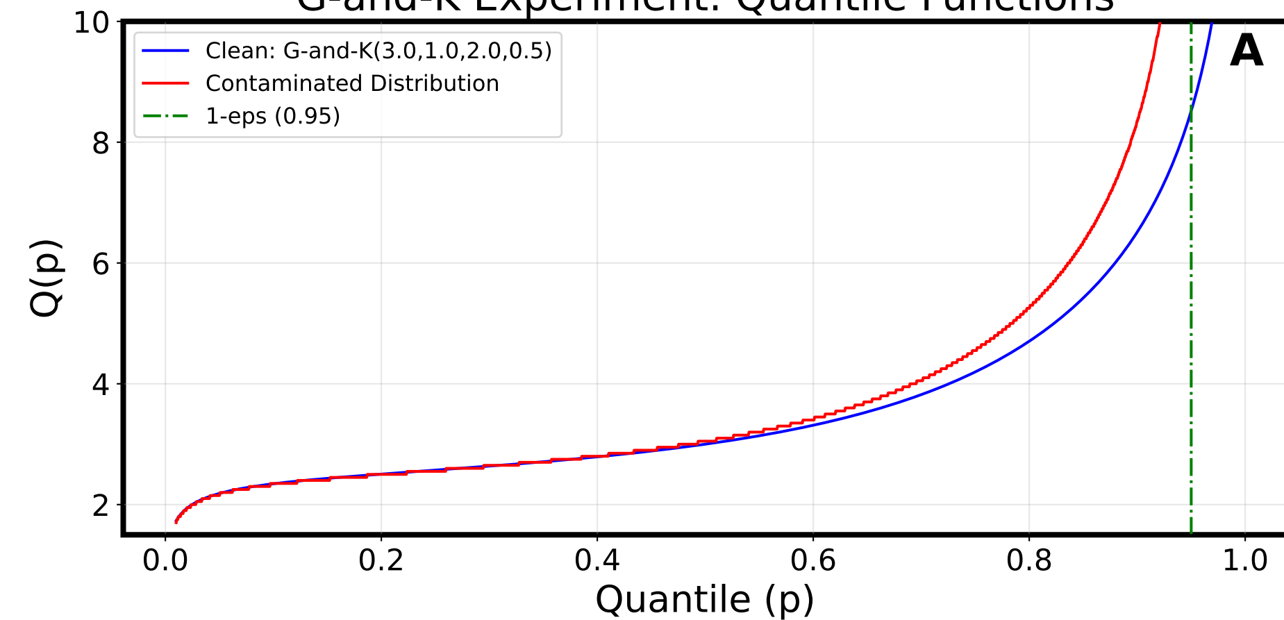
G-and-K Experiment: Quantile Functions
