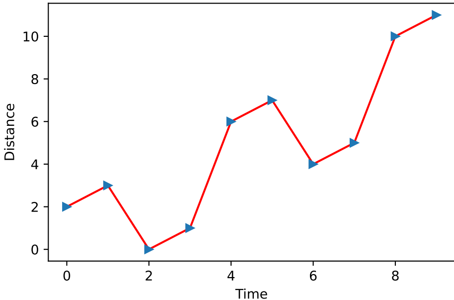
Graph Drawing
