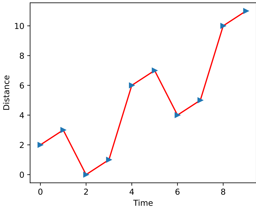
Graph Drawing
