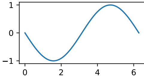
-\sin(x)
