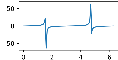
\tan(x)
