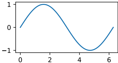
\sin(x)
