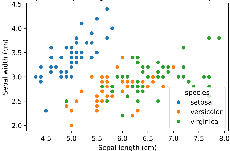
Scatter plot of sepal length and width with the hue parameter
