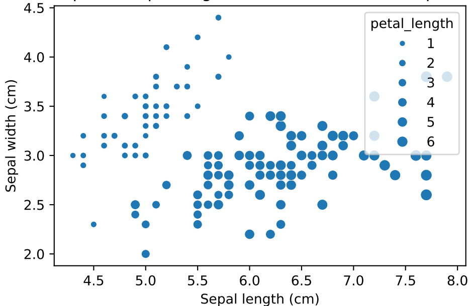
Scatter plot of sepal length and width with the size parameter
