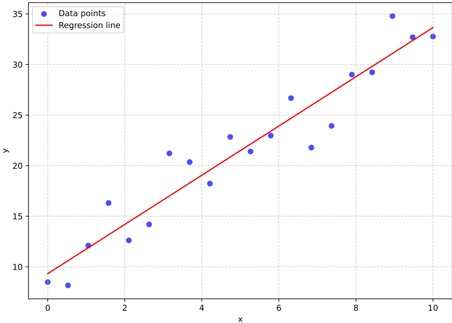
Linear regression using numpy.polyfit
