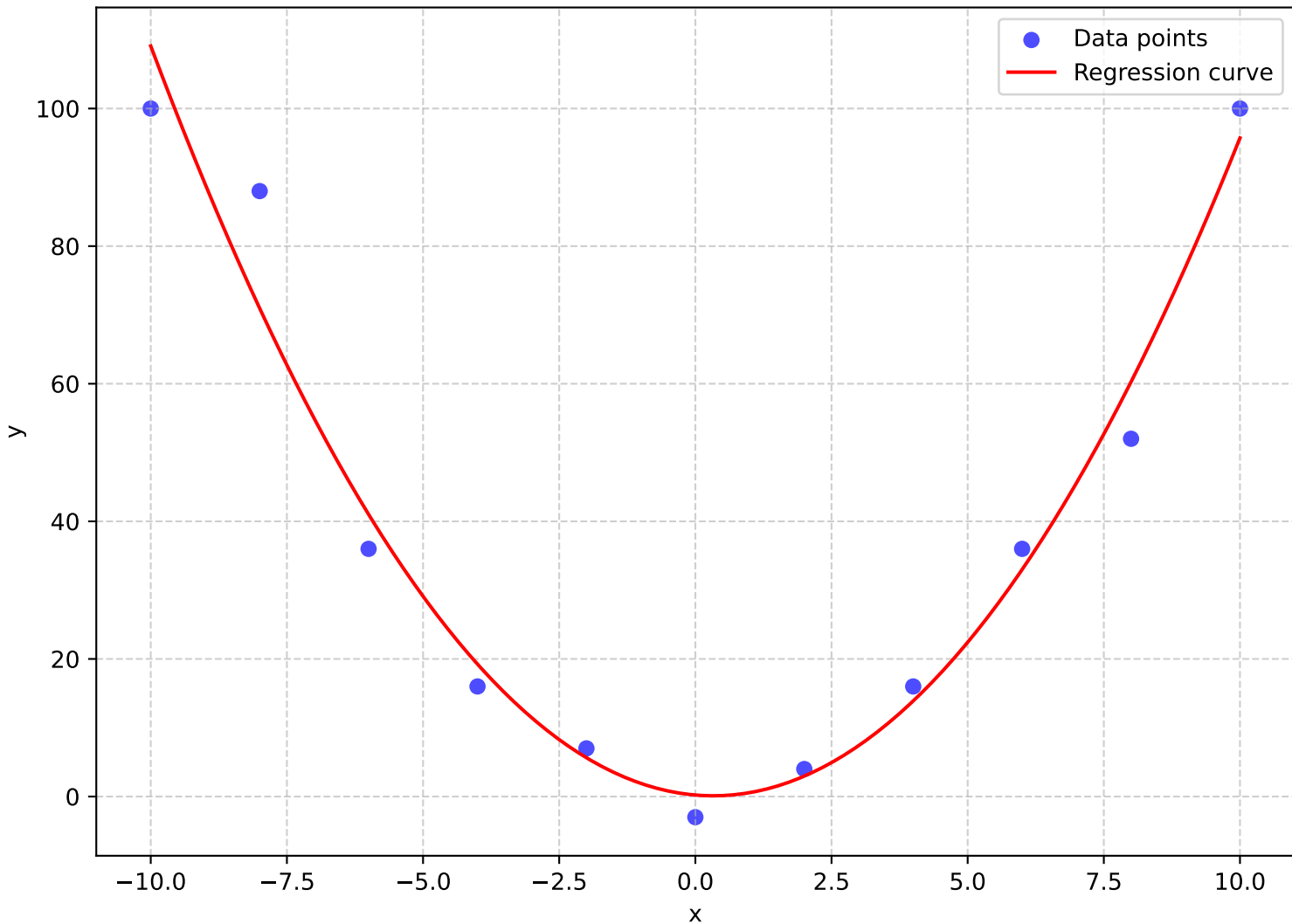
Quadratic regression using numpy.polyfit
