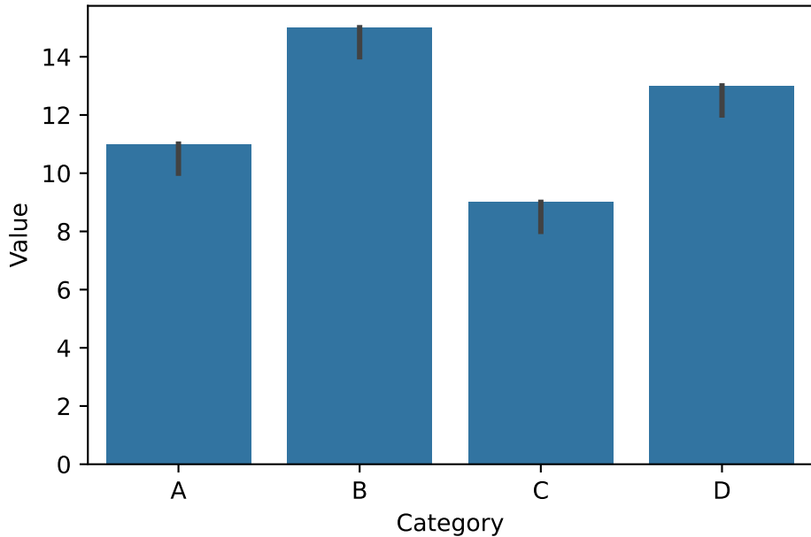
Bar chart with 'estimator=max'
