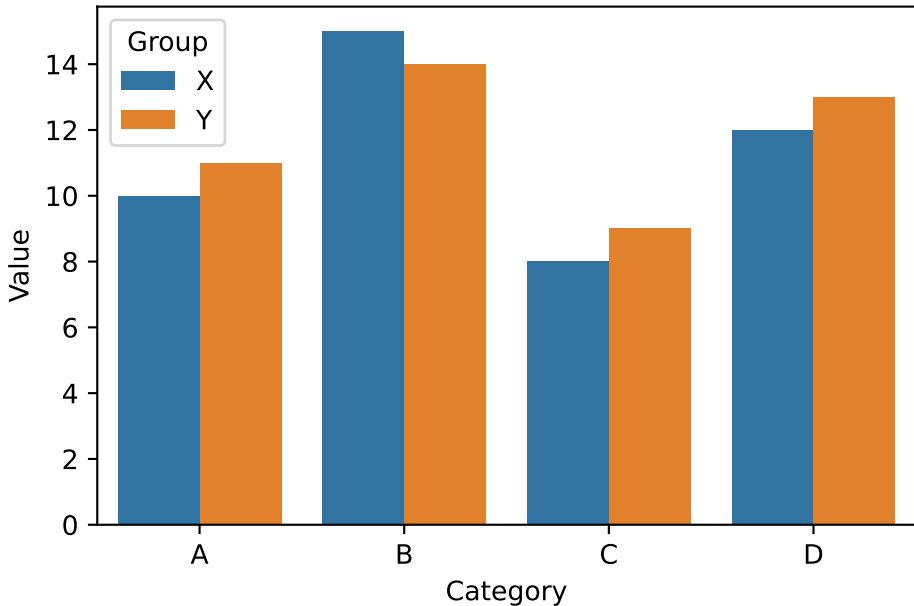
Bar chart with 'hue=Group'
