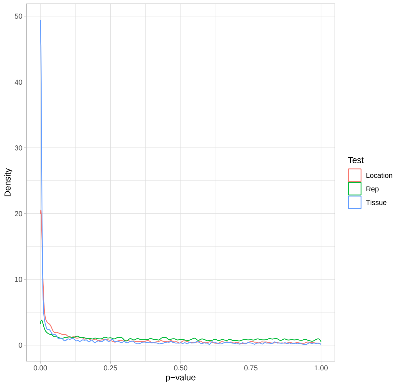
Density plot
