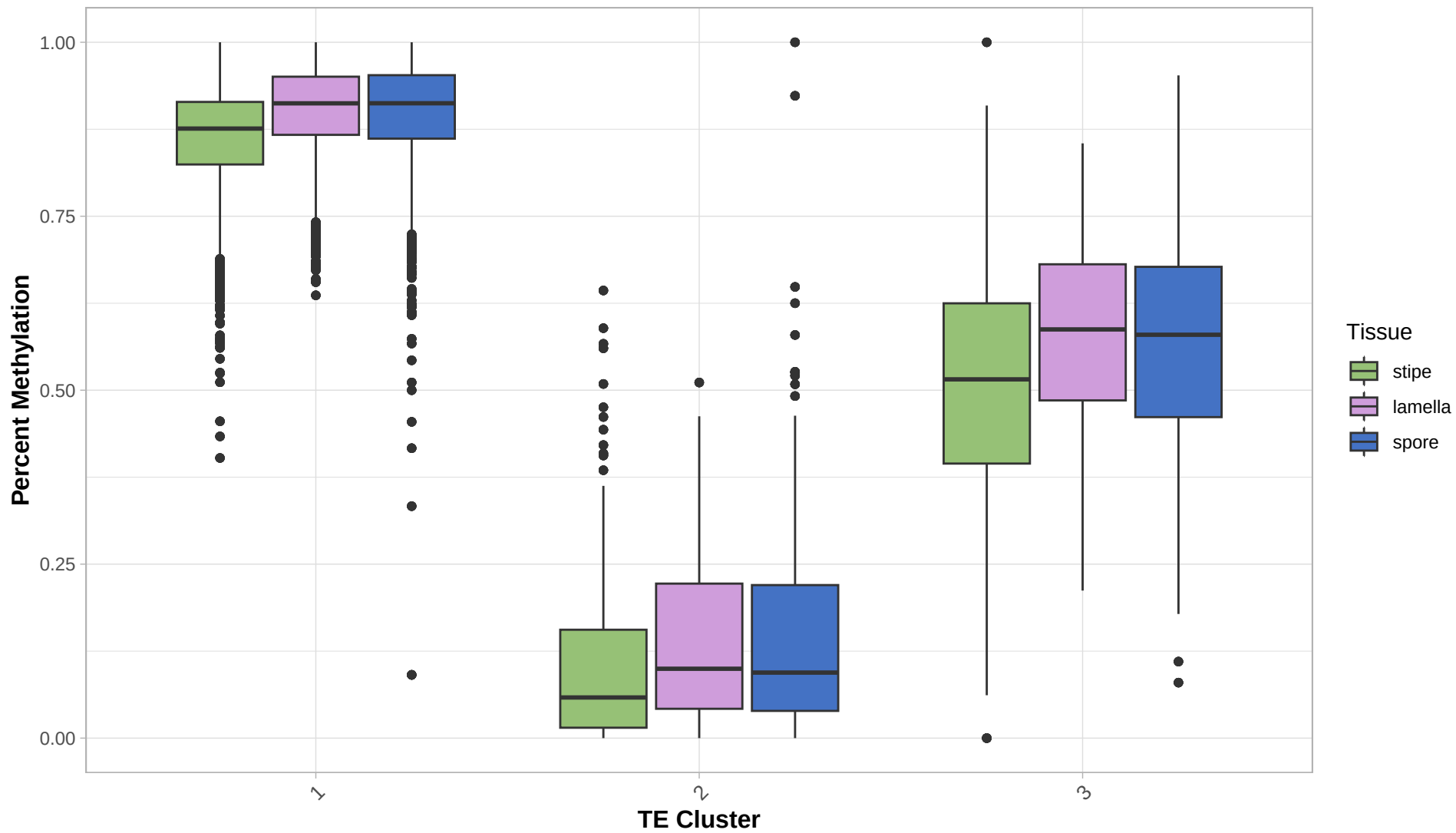
Methylation levels per TE cluster
