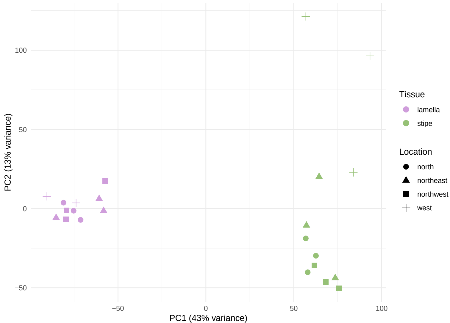
PCA of VST-normalized counts
