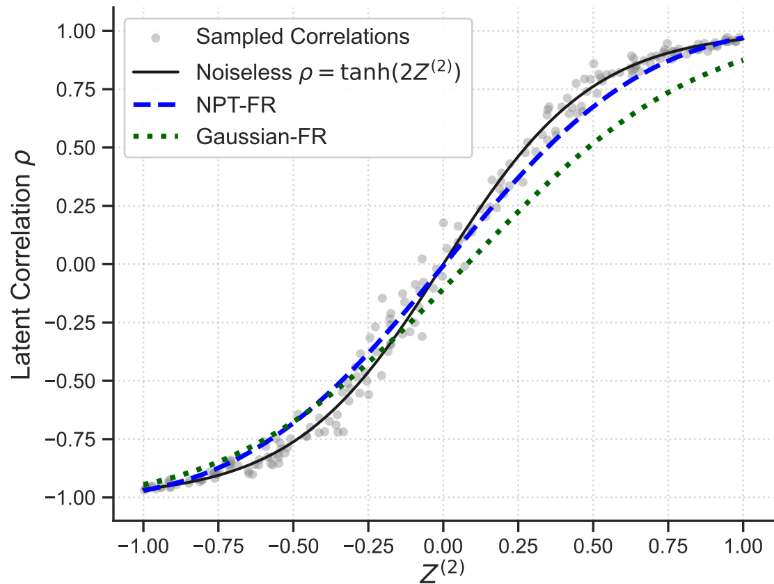
Nonlinear Correlation Structure
