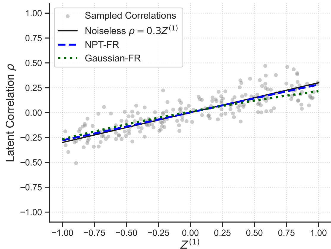
Linear Correlation Structure
