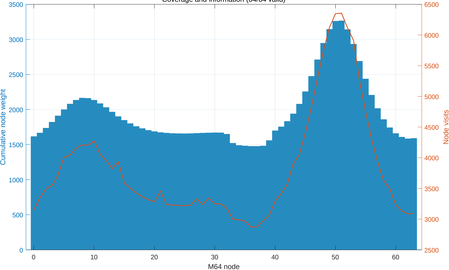
Coverage and information (64/64 valid)
