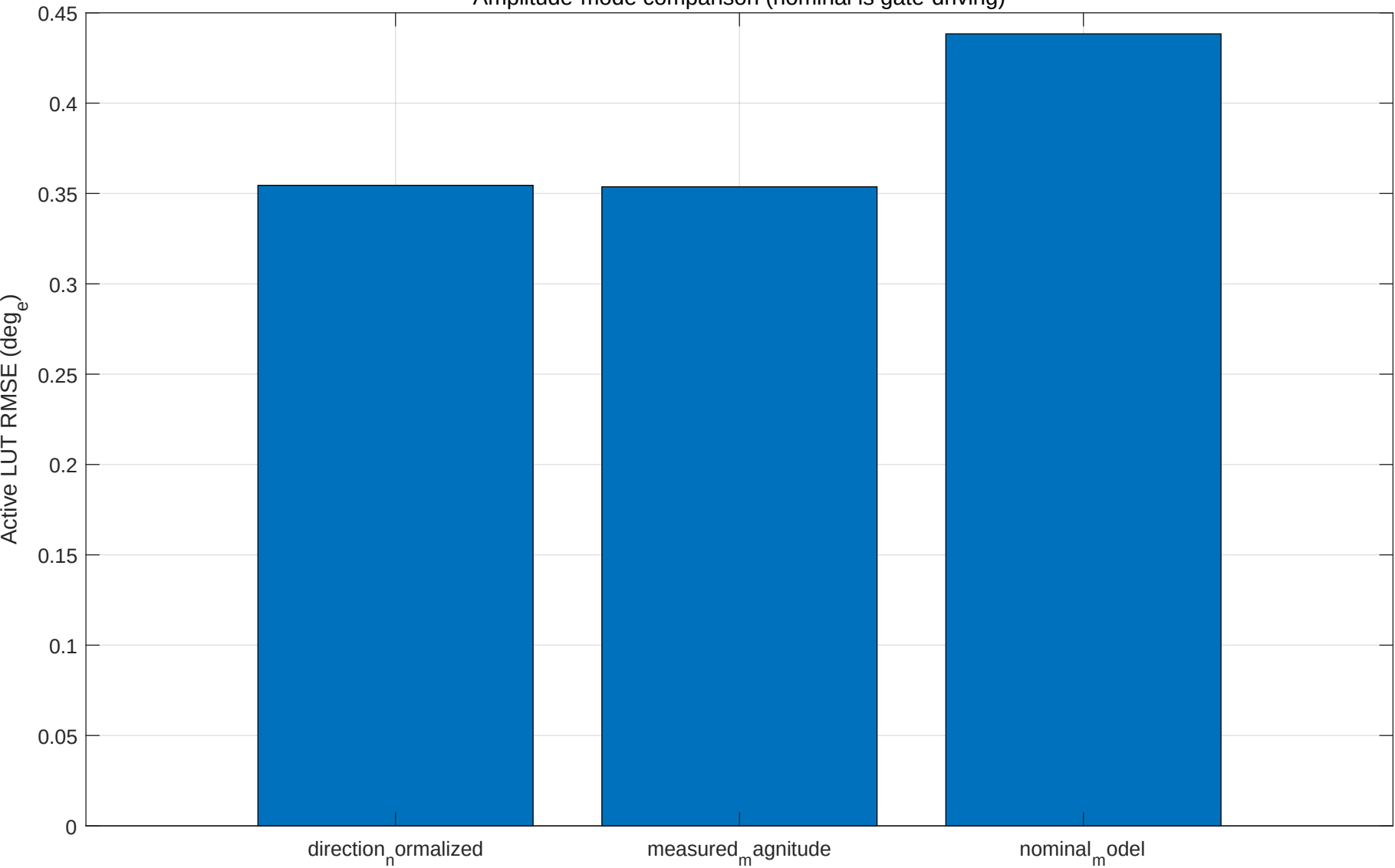
Amplitude-mode comparison (nominal is gate-driving)
