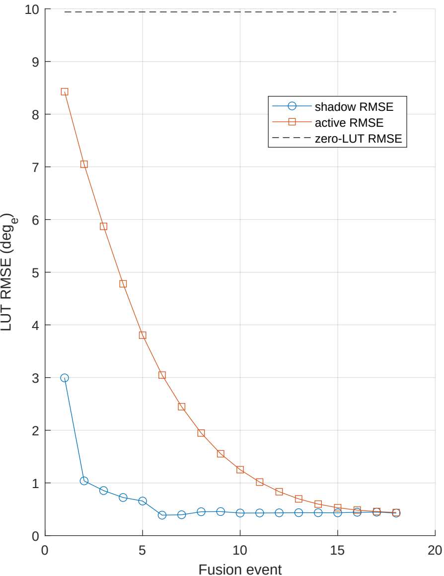
LUT learning evolution — improvement should rise and then settle
