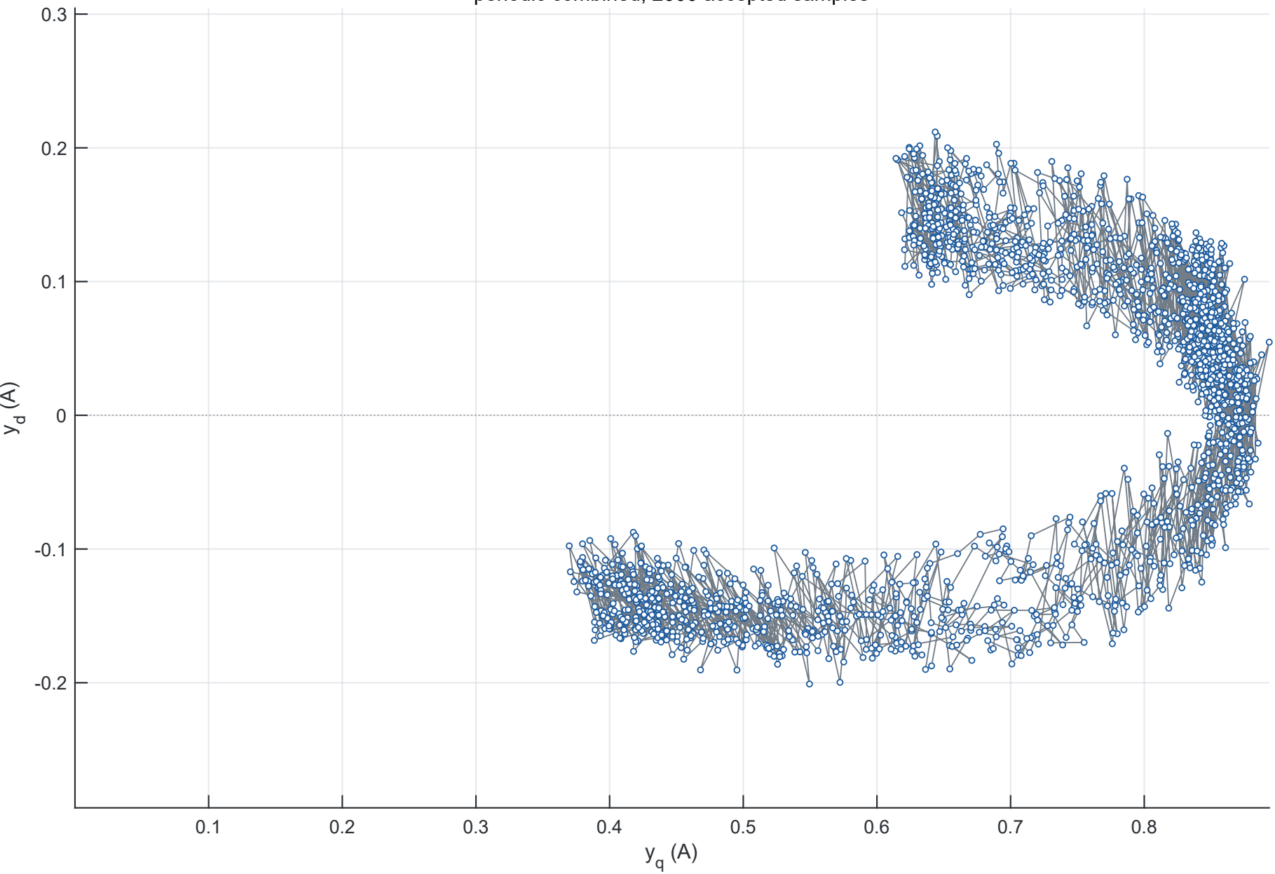
Direction-normalized residual trajectory periodic combined; 2000 accepted samples
