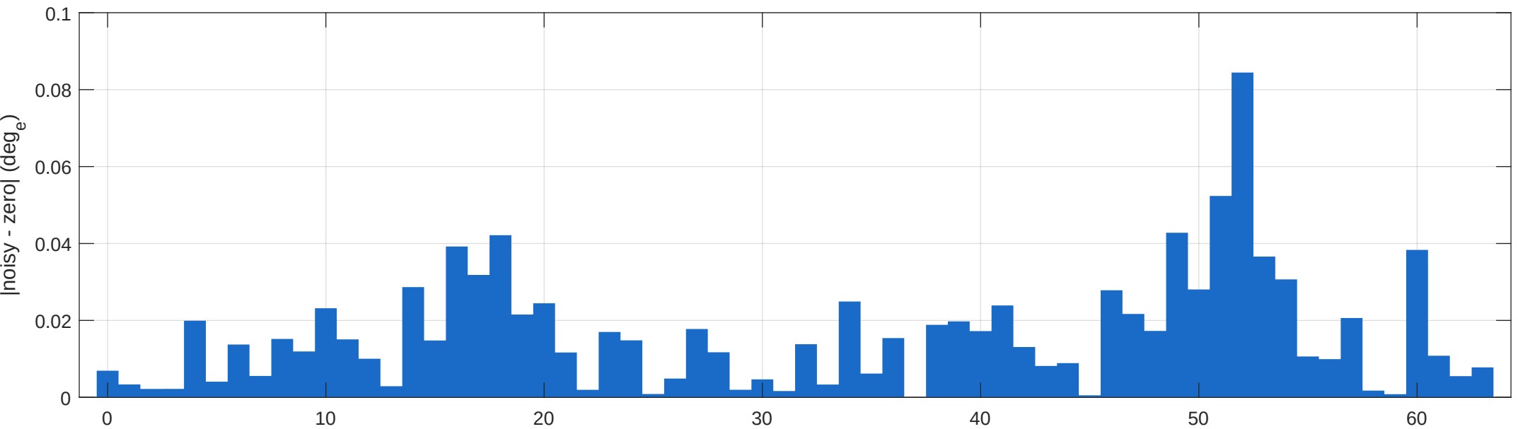
Per-node LUT noise floor
