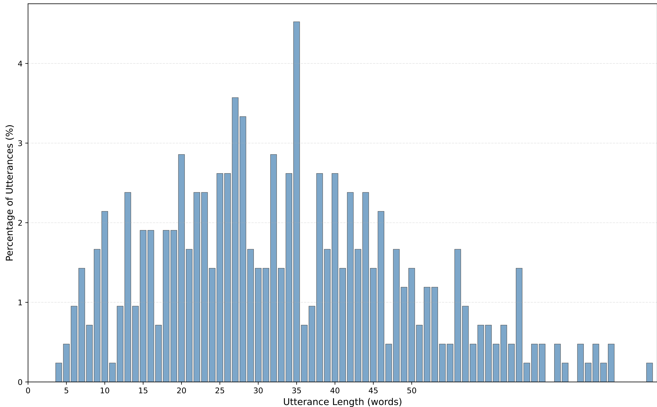
Utterances with Worsened WER After N-gram Incorporation
