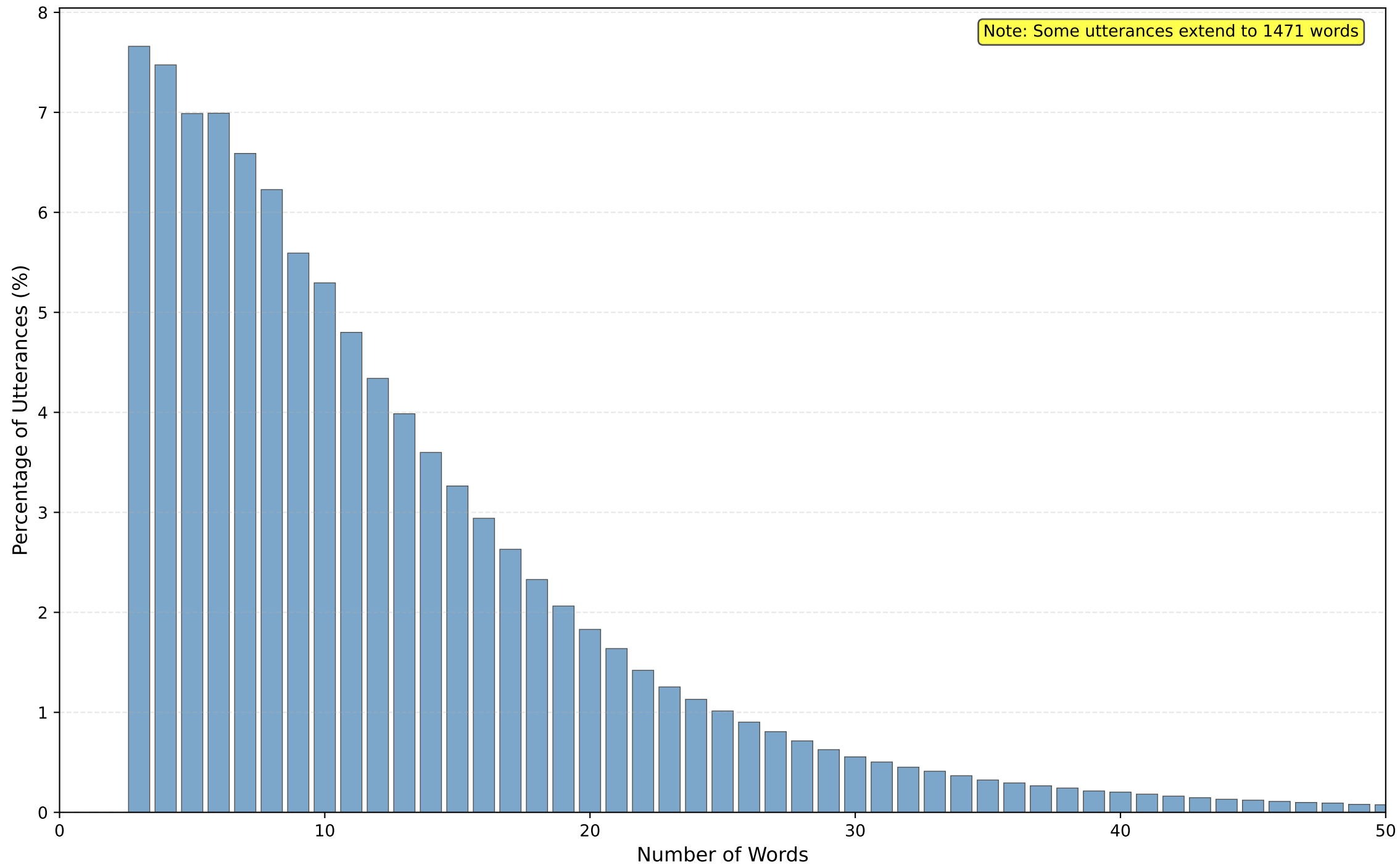
Distribution of Utterance Lengths (After Filtering)
