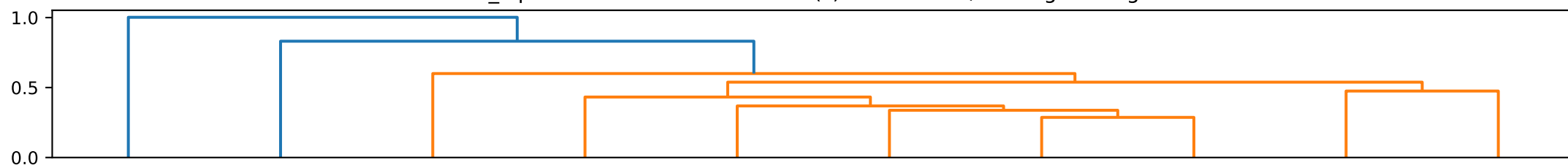
B_alpha1 · fixed structural block(s) · Euclidean / average linkage
