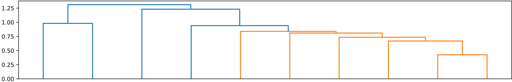
E · fixed structural block(s) · Euclidean / average linkage
