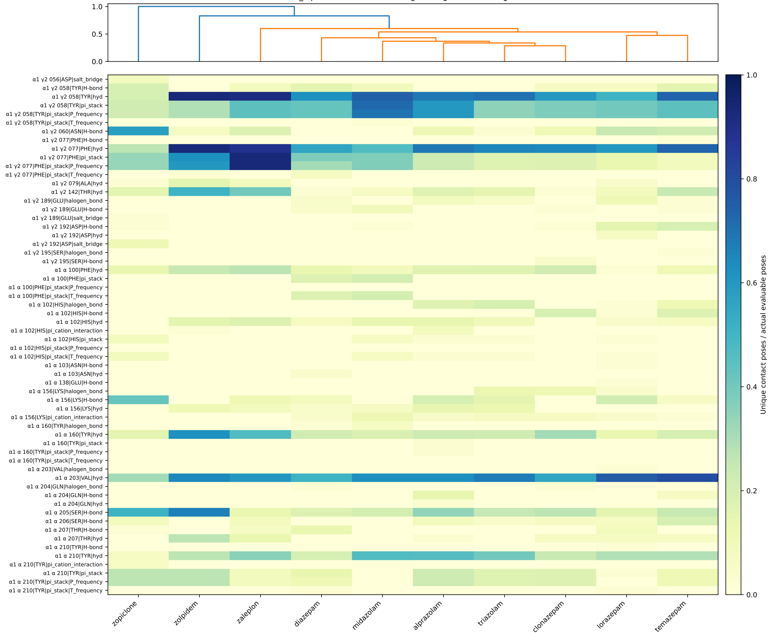
B_alpha1 · Euclidean / average linkage · frozen drug order
