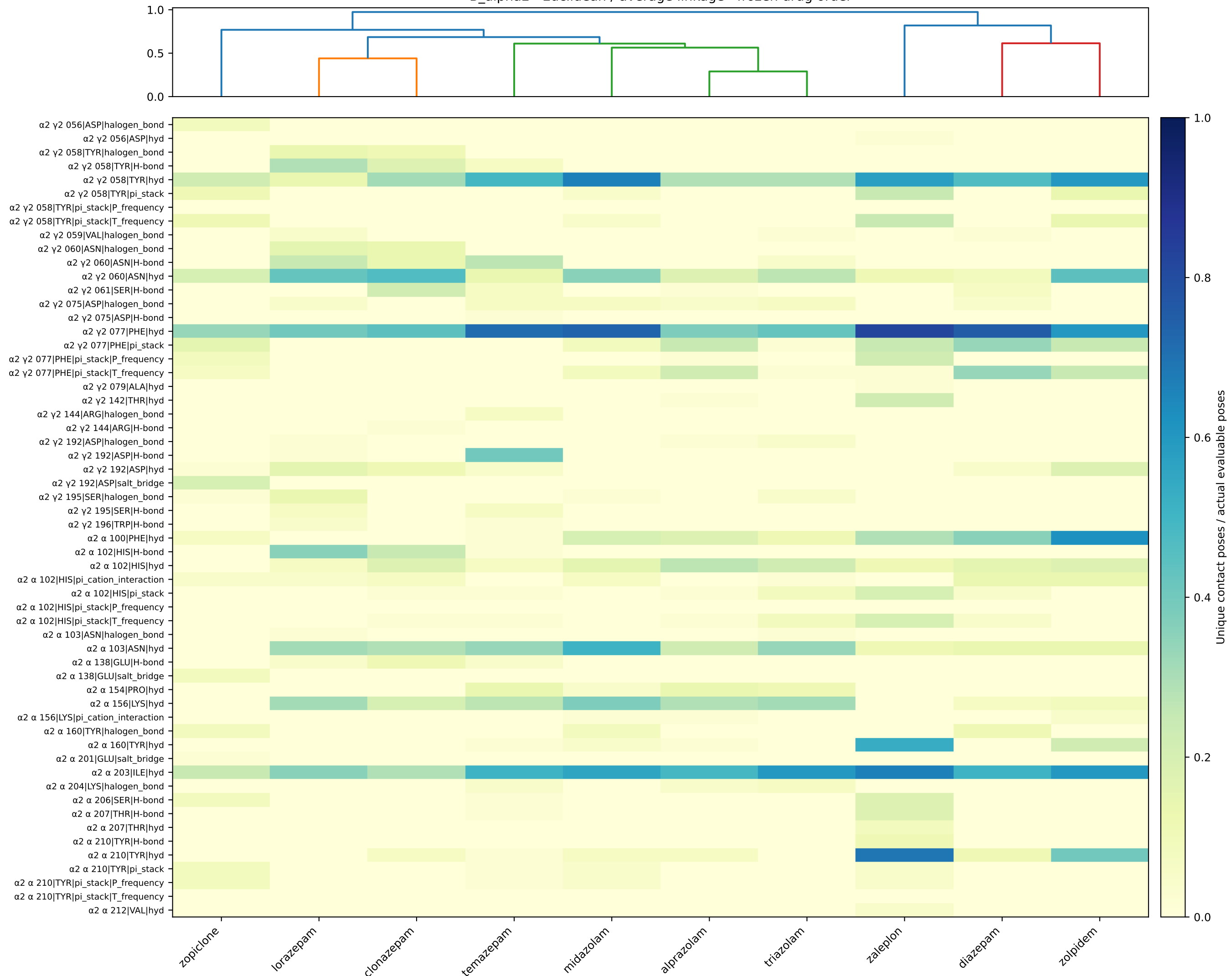
B_alpha2 · Euclidean / average linkage · frozen drug order
