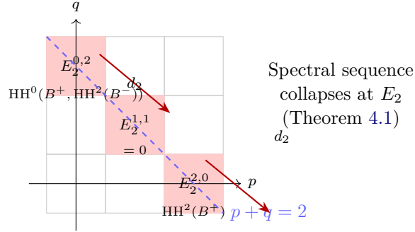
FIGURE 2. The E_2 page of the Drinfeld double spectral sequence in total degree p + q = 2 . The three terms E_2^{0,2}, E_2^{1,1}, E_2^{2,0} are shown; E_2^{1,1} = 0 by \text{HH}^1(B^-) = 0 (Lemma 4.2), and the differentials d_2, d_r ( r \geq 3 ) vanish by the first-quadrant condition.
