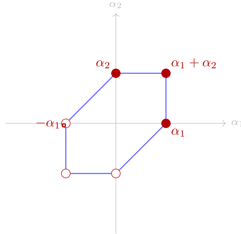
FIGURE 5. The A_2 root system. The three positive roots \alpha_1, \alpha_2, \alpha_1 + \alpha_2 give |\Phi^+| = 3 ; combined with \text{rank}(\mathfrak{sl}_3) = 2 , the formula \dim \text{HH}^2 = \text{rank} + 2|\Phi^+| = 2 + 6 = 8 is verified at \ell = 3 .
