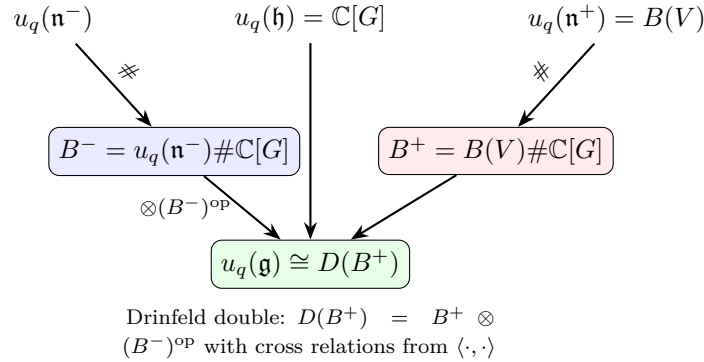
FIGURE 1. Triangular decomposition of u_q(\mathfrak{g}) and the Drinfeld double structure. The Cartan part u_q(\mathfrak{h}) = \mathbb{C}[G] is shared between B^+ and B^- ; the Nichols algebras B(V) = u_q(\mathfrak{n}^+) and u_q(\mathfrak{n}^-) are dual via the Hopf pairing.
