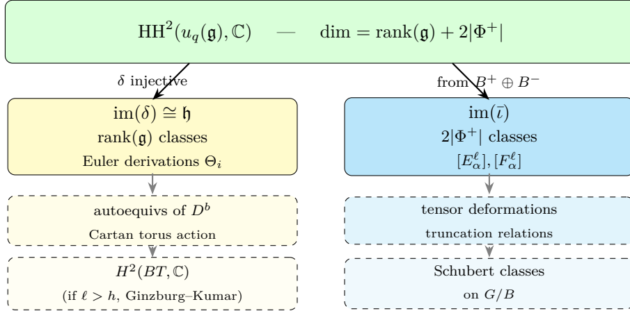
FIGURE 4. Decomposition of \mathrm{HH}^2(u_q(\mathfrak{g}), \mathbb{C}) into the \mathrm{rank}(\mathfrak{g}) Cartan-type classes (left) and the 2|\Phi^+| \ell -th power classes (right), with categorical and geometric interpretations. The algebraic and categorical levels are unconditional; the geometric level requires \ell > h .
