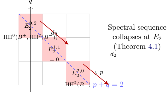
FIGURE 2. The E_2 page of the Drinfeld double spectral sequence in total degree p + q = 2 . The three terms E_2^{0,2}, E_2^{1,1}, E_2^{2,0} are shown; E_2^{1,1} = 0 by \mathrm{HH}^1(B^-) = 0 (Lemma 4.2), and the differentials d_2, d_r ( r \geq 3 ) vanish by the first-quadrant condition.
