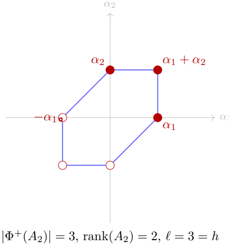
FIGURE 5. The A_2 root system. The three positive roots \alpha_1, \alpha_2, \alpha_1 + \alpha_2 give |\Phi^+| = 3 ; combined with \mathrm{rank}(\mathfrak{sl}_3) = 2 , the formula \dim \mathrm{HH}^2 = \mathrm{rank} + 2|\Phi^+| = 2 + 6 = 8 is verified at \ell = 3 .
