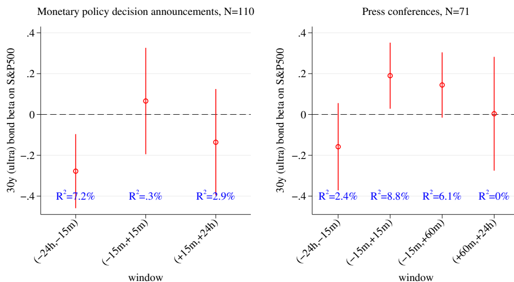
Figure E.2. Bond betas. The figure presents betas of 30-year Treasury ultra bond futures returns on S&P 500 E-mini futures returns in different windows around scheduled FOMC announcements and press conferences. Robust 95% confidence intervals are included.
