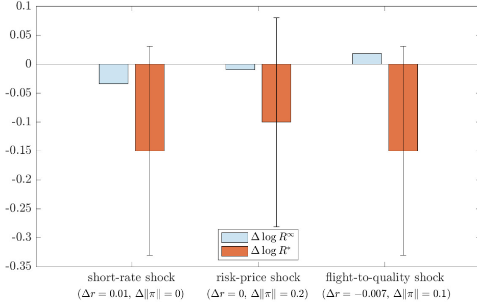
Figure 5. Shock exposures of key returns. The figure presents the responses of the growth-optimal portfolio return \log R_t^* and the long bond return \log R_t^\infty to a one standard deviation shock in each of the three shocks. The bars represent the average responses, while the thin error bands represent [-1, +1] standard deviations of the response.
