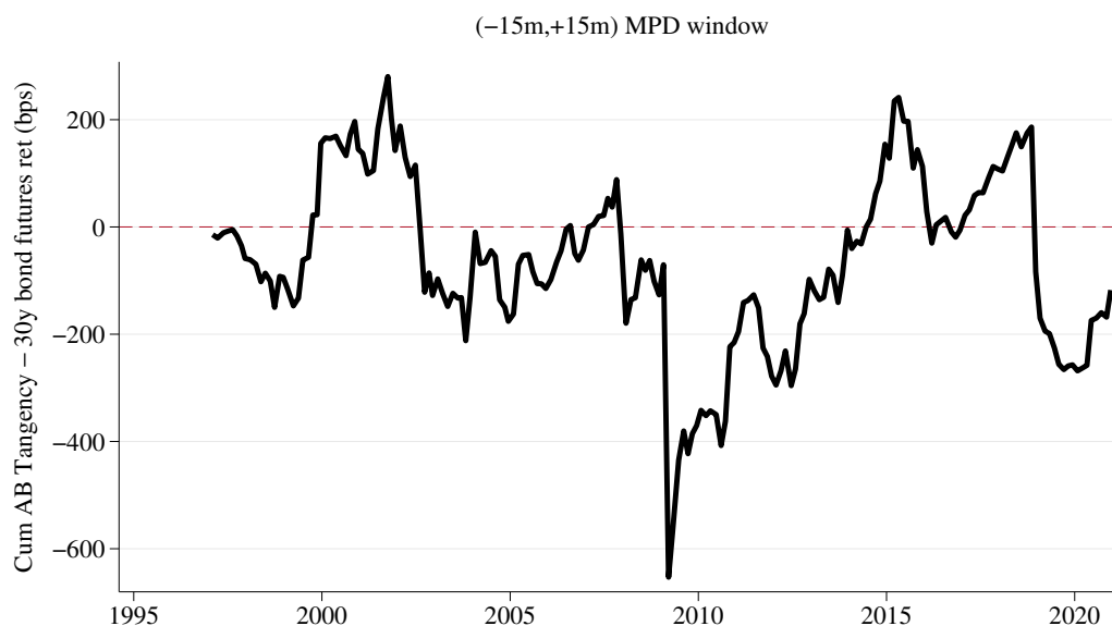
Figure E.3. Cumulative returns in a narrow window around FOMC policy announcements. The figure plots cumulative log returns on a long-short portfolio of Aletti-Bollerslev (AB) tangency portfolio in excess of 30-year Treasury bond futures. The returns are calculated from -15 to +15 minutes around scheduled FOMC announcements. The sample period covers 191 meetings from 1997:02 through 2020:12.
