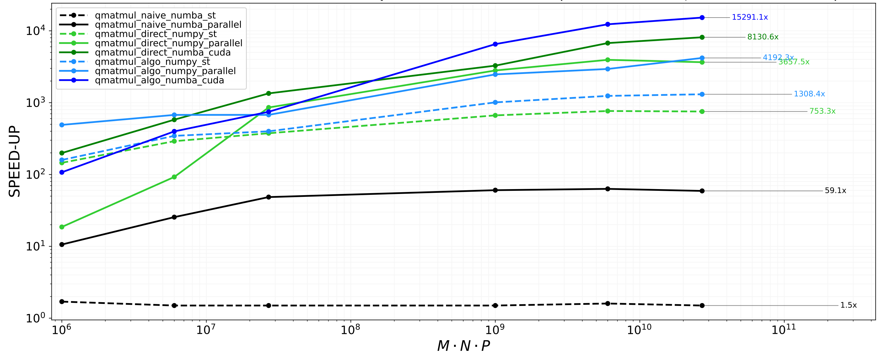
LOG-LOG PLOT OF SPEED-UPS FOR QMATMUL FUNCTIONS (TYPE: FLOAT32, ENVIRONMENT: 2)
