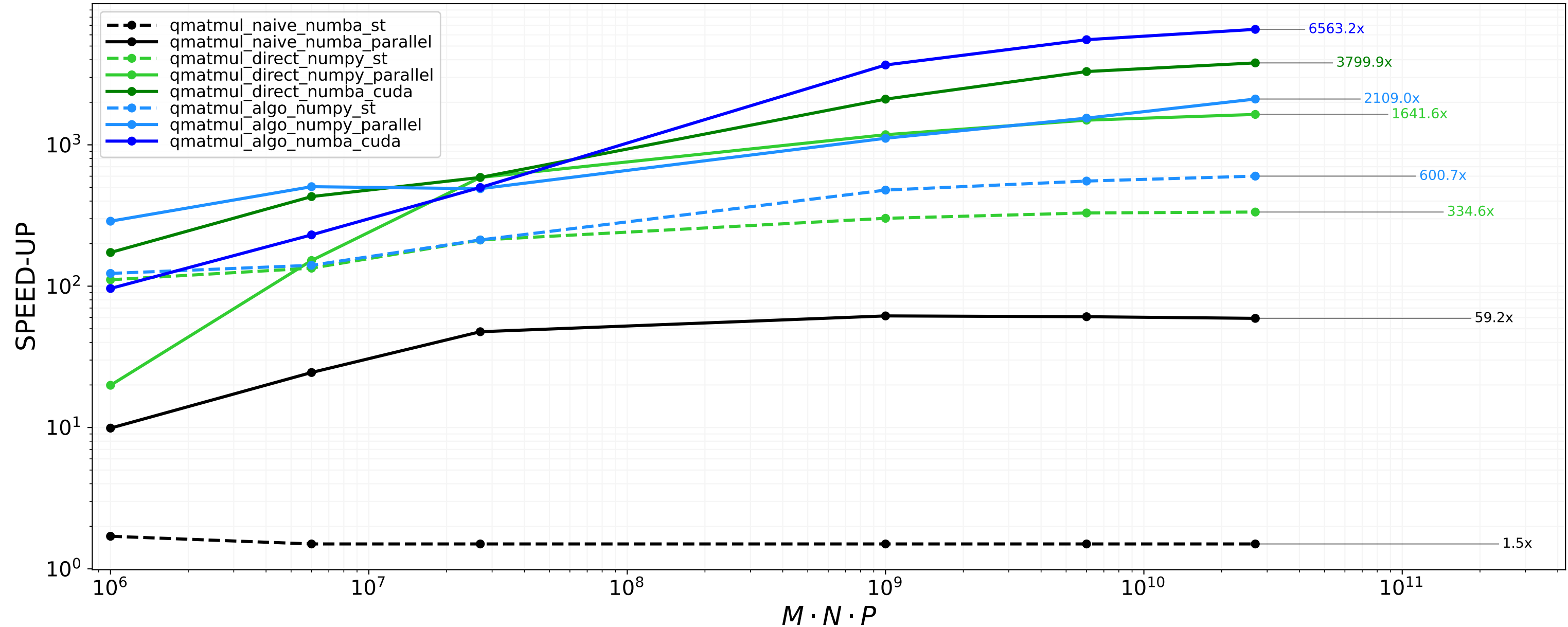
LOG-LOG PLOT OF SPEED-UPS FOR QMATMUL FUNCTIONS (TYPE: FLOAT64, ENVIRONMENT: 2)
