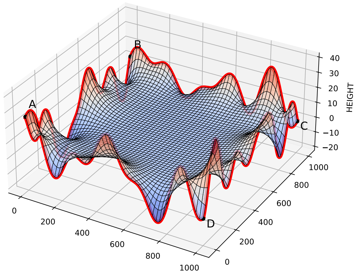
SHAPE COMPUTED BY: sfwf_contraction_cuda_large_atomicmax [ d_\infty : 9.918e-05, iterations: 37400]
