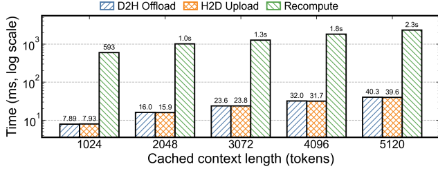
Figure 17. D2H offload, H2D upload, and recomputation time for Qwen2.5-14B on A100 PCIe.
