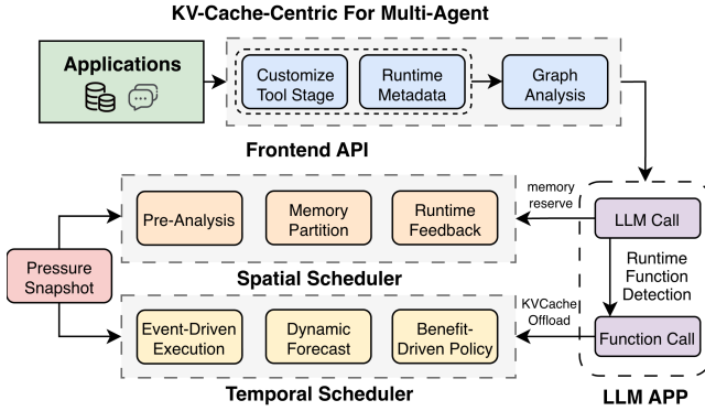
Figure 4. TokenCake Overview.
