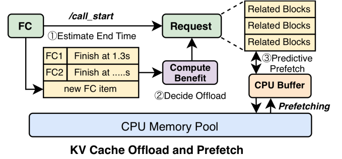
Figure 7. Lifecycle of the Temporal Scheduler’s offload and predictive upload mechanism.
