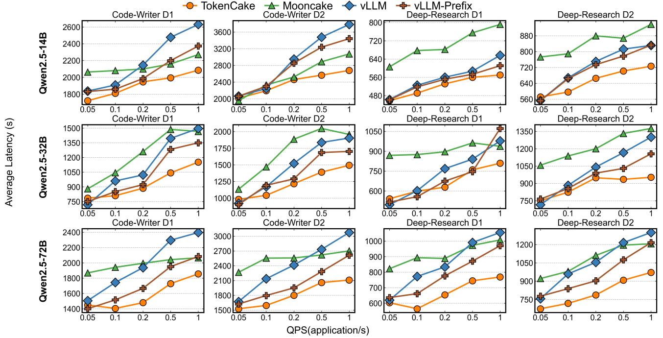
Figure 9. End-to-end application latency comparison of TokenCake, vLLM, vLLM-Prefix, and Mooncake. Each chart plots average latency against queries-per-second (QPS) for the specified application, model, and dataset.
