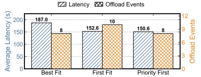
Figure 15. Average latency (left axis) and offload event count (right axis) for three request-selection policies.
