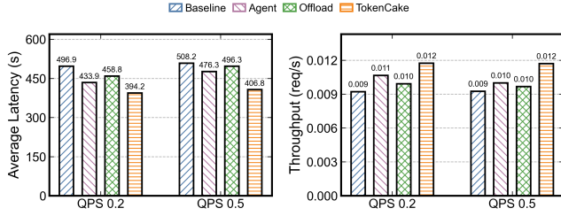
Figure 11. Component behavior at 0.2 and 0.5 QPS (Qwen2.5-14B Code-Writer, 20 apps, 0.5 GPU memory utilization).
