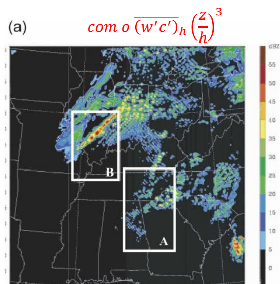
maximum (dBZ) at (a) 1800 UTC (b) 10 Nov 2002
