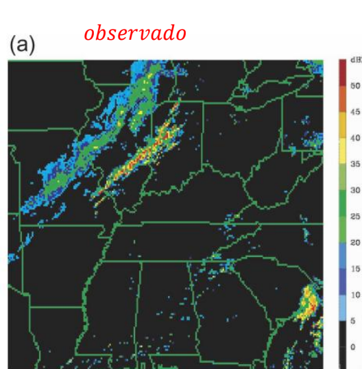
maximum (dBZ) at (a) 1800 UTC 10 Nov 2002
