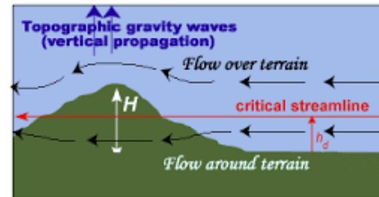
Parameterized Sub-grid Scale Flow Over Topography
