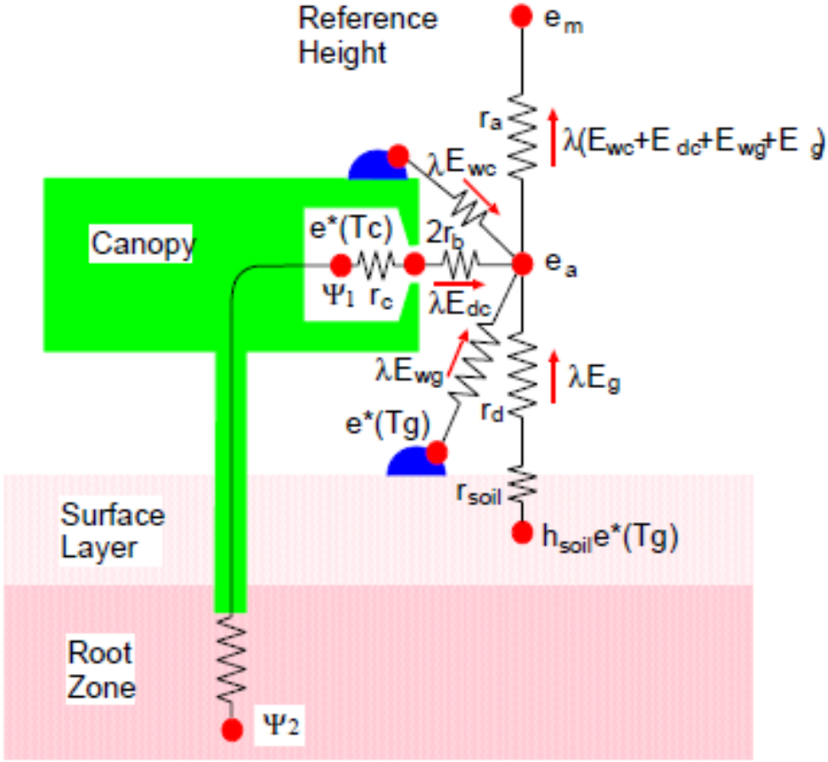
(b) Latent heat flux
