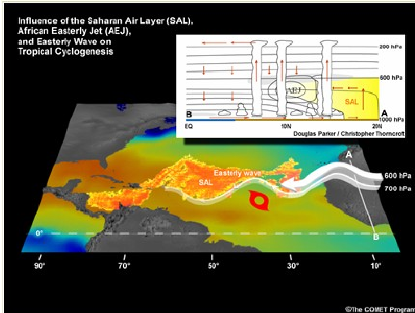
Fig. 8.56. Schematic of the Saharan Air Layer, and influences on genesis, as described by Dunion and Velden 152 and Karyampudi and Pierce. 153 The African easterly jet (AEJ) at the southern bound of the SAL and an African easterly wave are shown. The cross-section is a conceptual model of the SAL, AEJ, and convective weather systems based on the JET 2000 field program.
