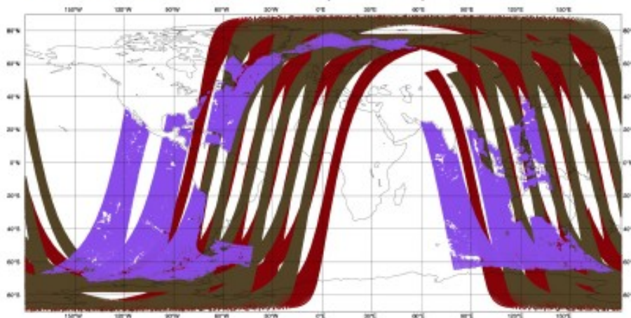
Scatterometer data (535,183)
