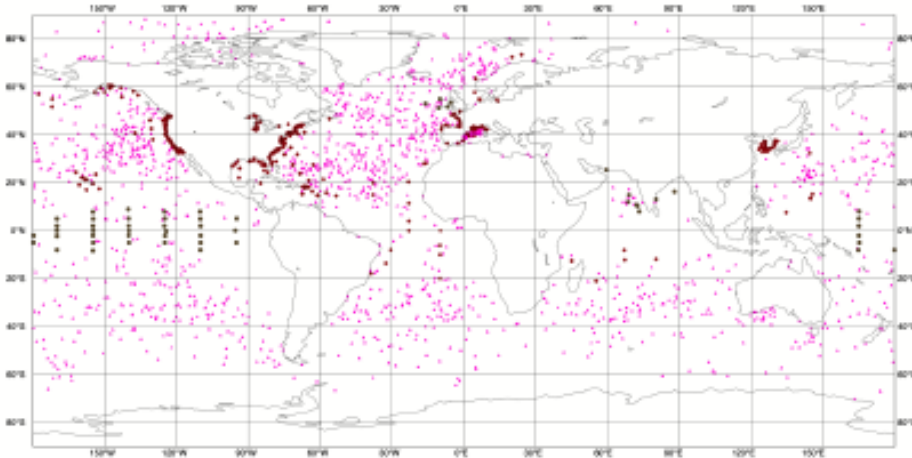
Buoy data (1,940)
