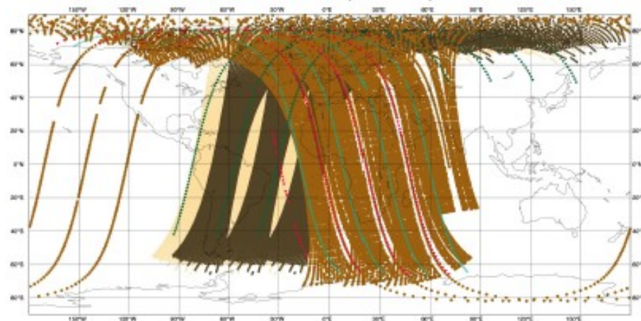
Ozone observations (60,189)
