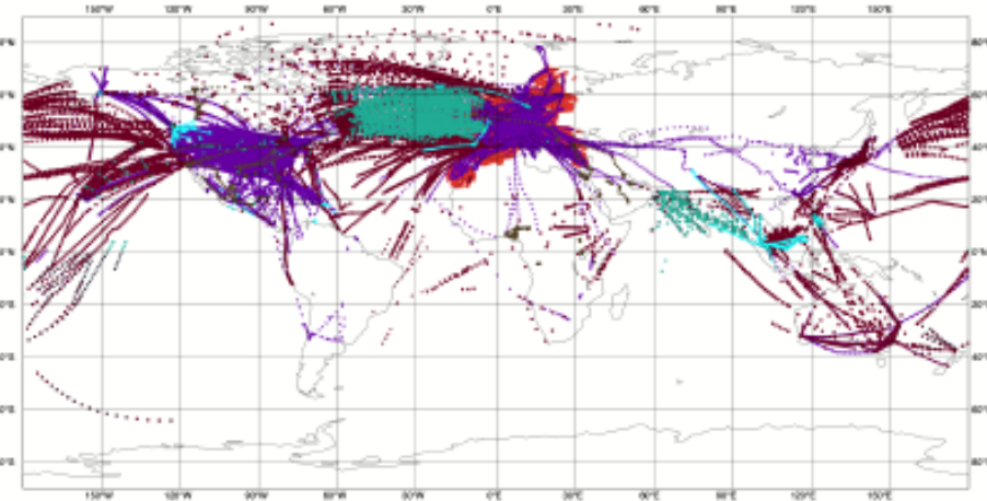
Aircraft observations (1,850,685)
