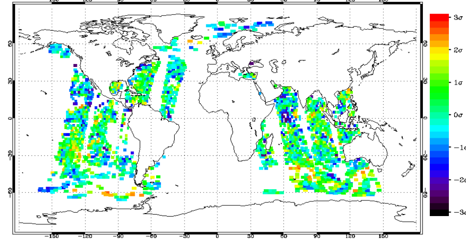
Date = 2008070112 DMSP-13/14/15 Brightness temperature O-P
