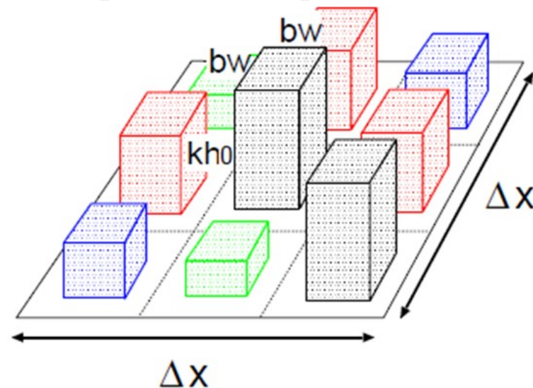
Figure 2.5: Roof height distribution
