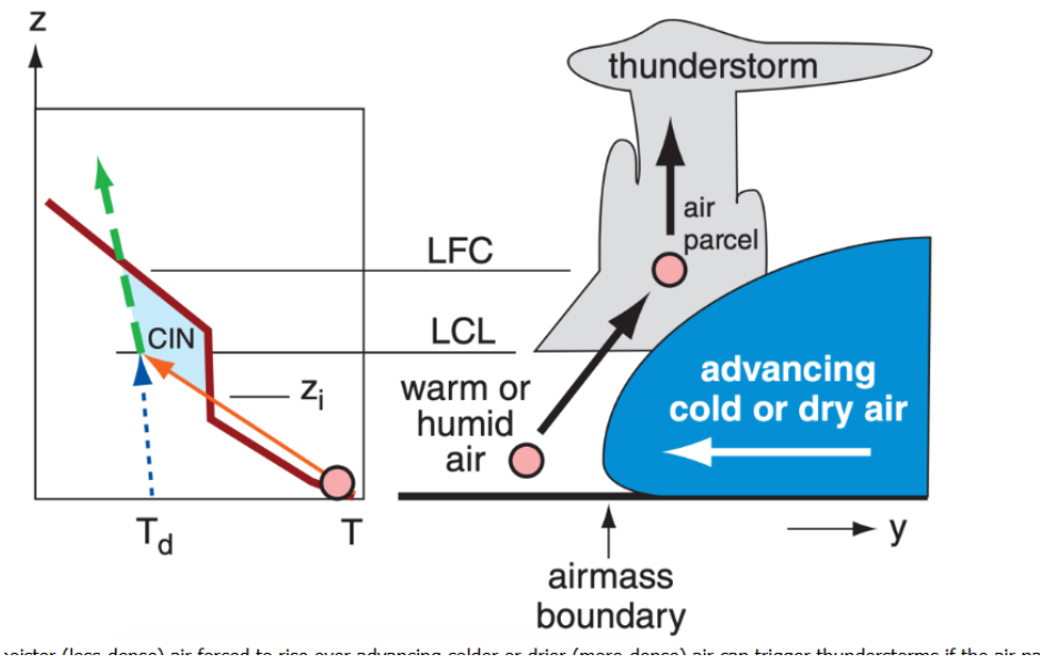
winter (less dense) air forced to rise over advancing colder or drier (more dense) air can trigger thunderstorms if the air is
