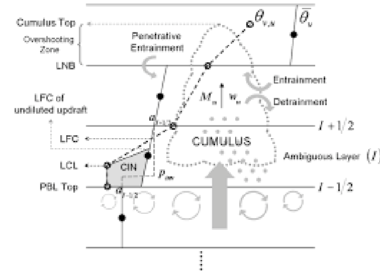
Fig. 4. Schematic diagram of a cumulus cloud showing the vertical structure and the processes of entrainment and detrainment.
