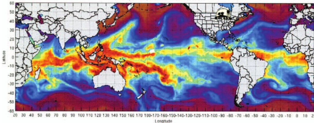
Morphed composite: 2009-01-25 00:00:00 UTC
